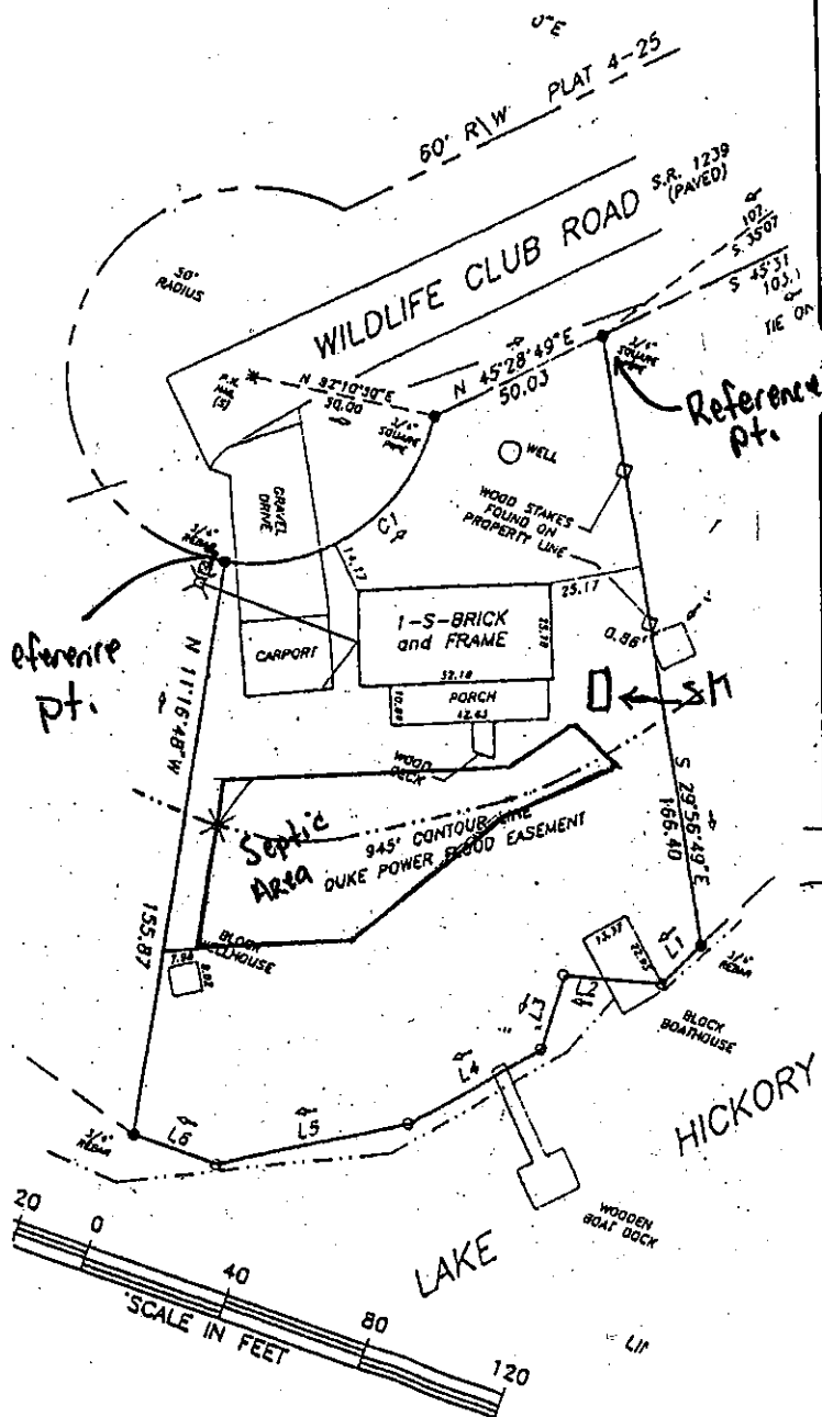
Advanced (Surveyed) Site Plan
